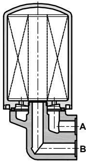
Sub-plate type, with top mounted element
