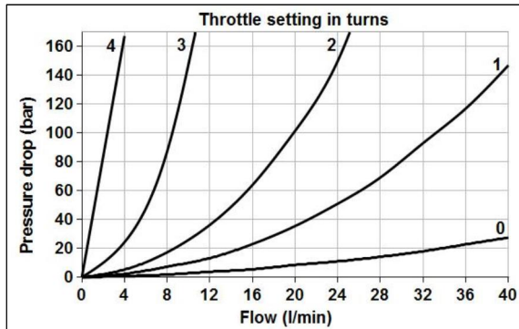
Pressure drop related to flow at throttle setting in turns, from throttle fully open condition to towards close.
